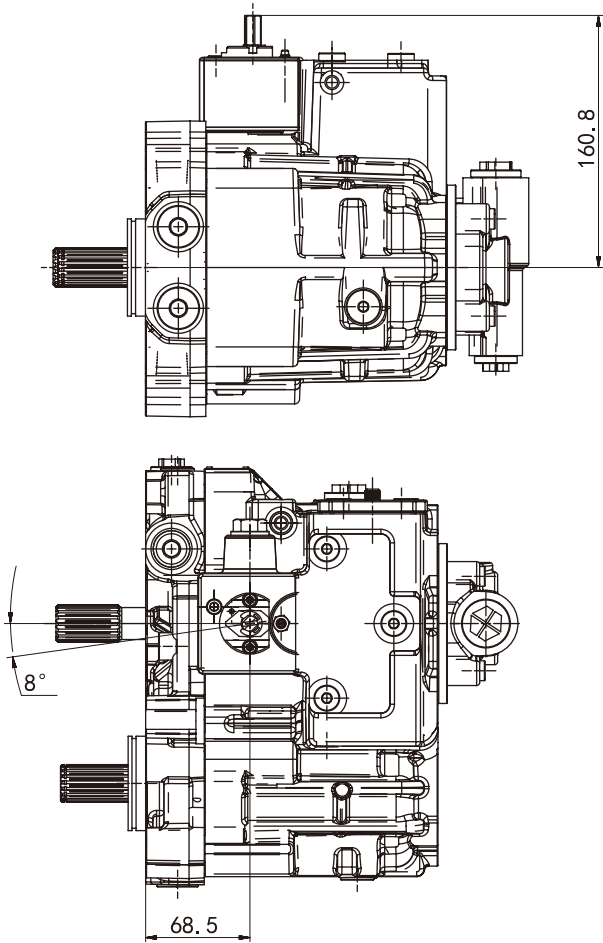
Mechanical servo control, with hex shaft without hand lever
