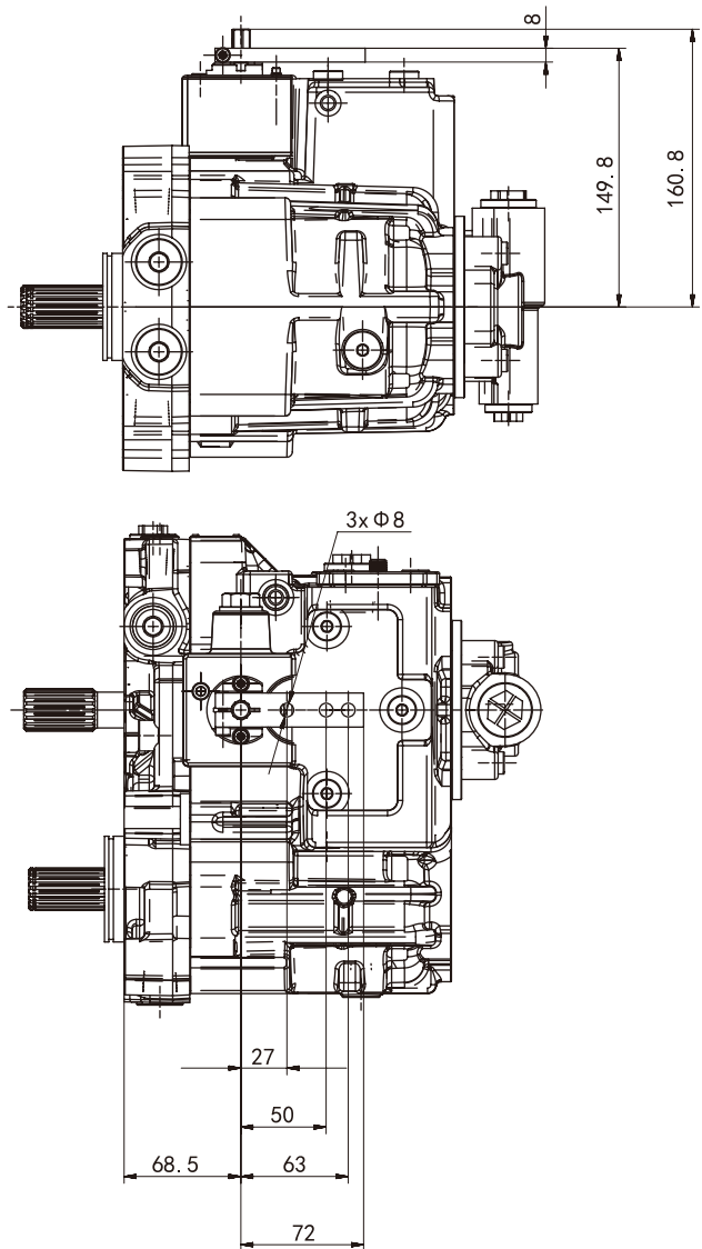
Mechanical servo control, with hex shaft with cross handle
