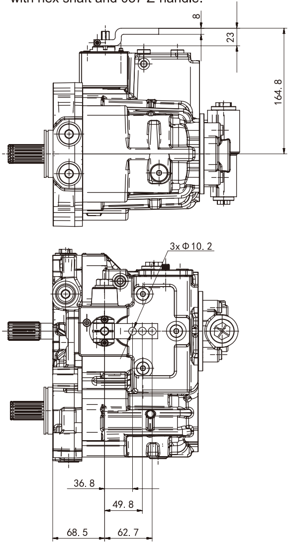
Mechanical servo control, with hex shaft and 037 Z-handle.
