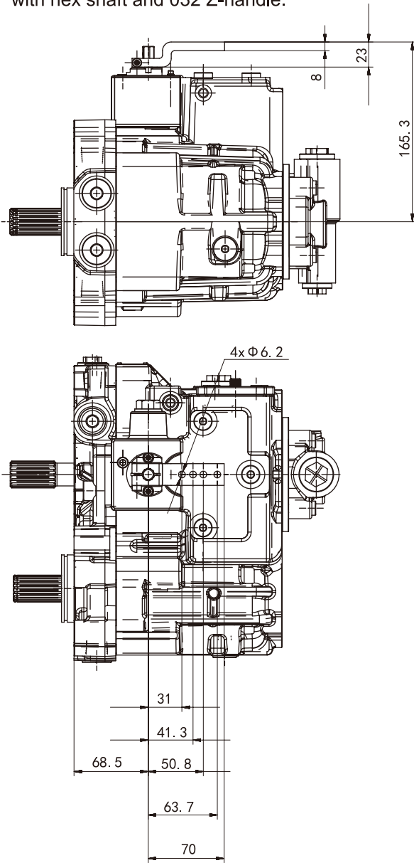
Mechanical servo control, with hex shaft and 032 Z-handle.
