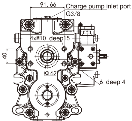
Front cover type F3
