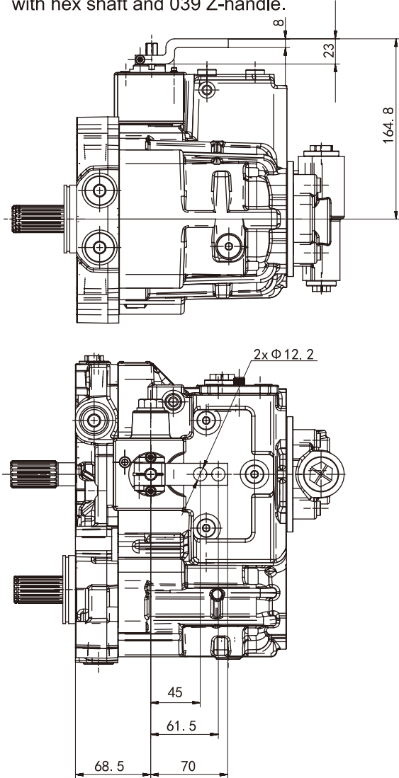
Mechanical servo control, with hex shaft and 039 Z-handle.
