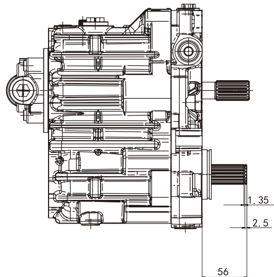
Motor shaft configuration J3
