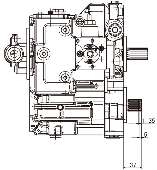
Motor shaft configuration J2
