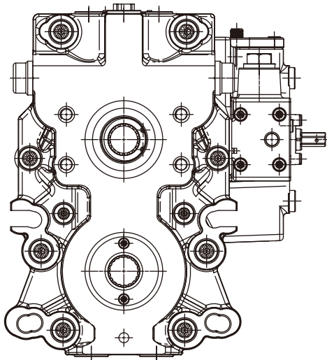
variable cylinder on the left
