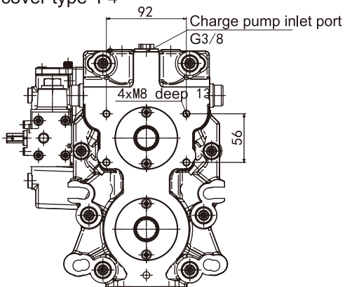
Front cover type F4
