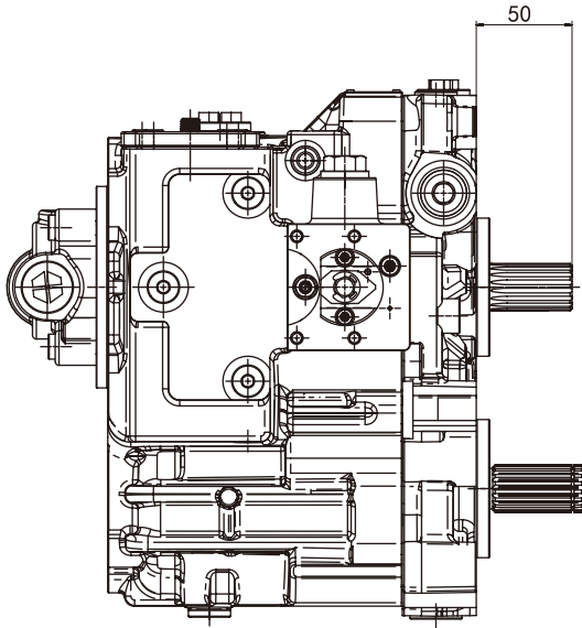
Pump shaft configuration J1
