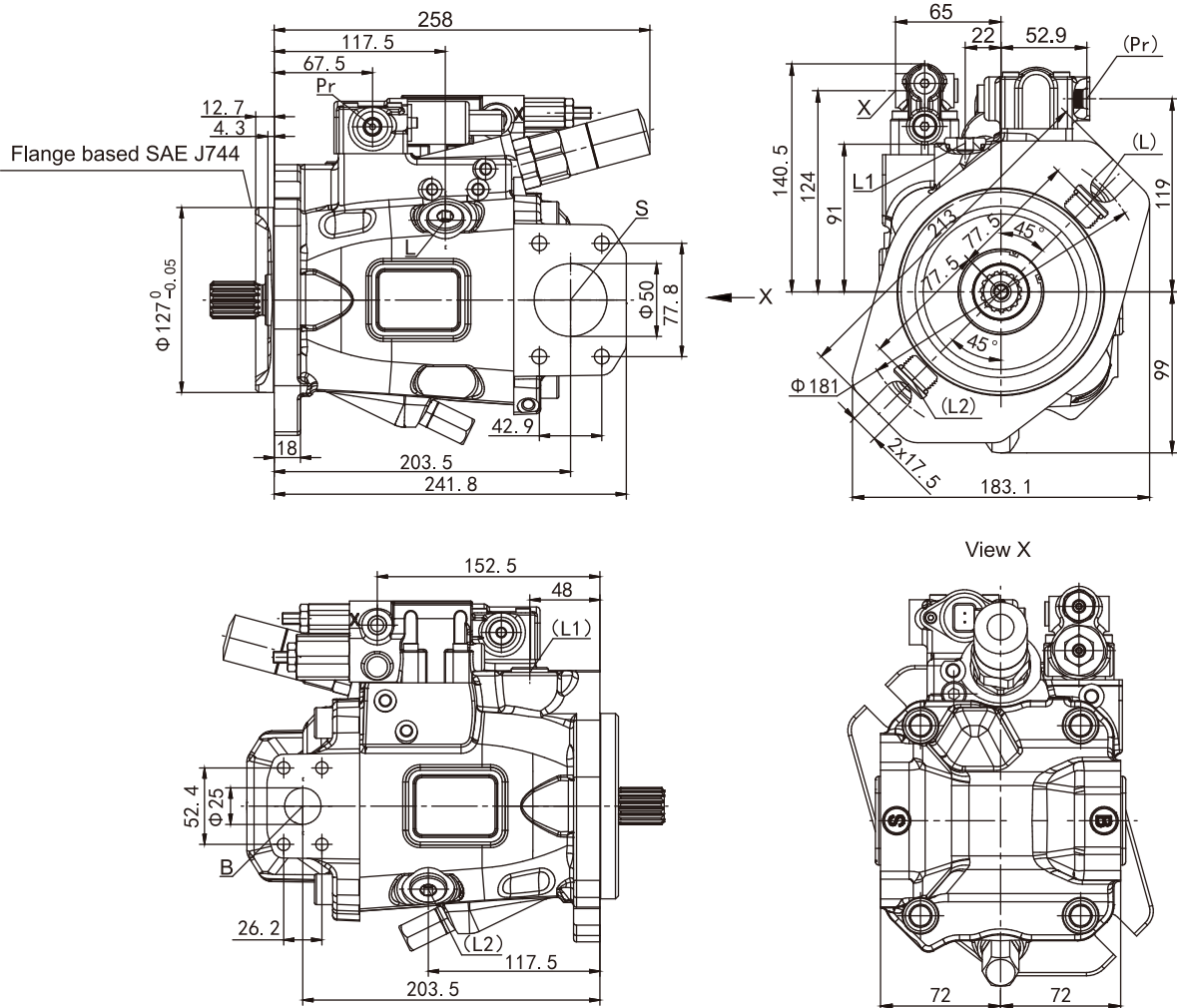
LE.DS-Electrically Proportional Power Control, clockwise rotation, mounting flange Z
