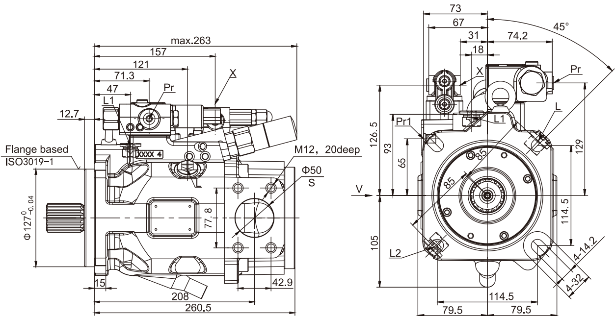
LEDS.-Pressure, Flow, Power controller, mounting flange D, series 01
