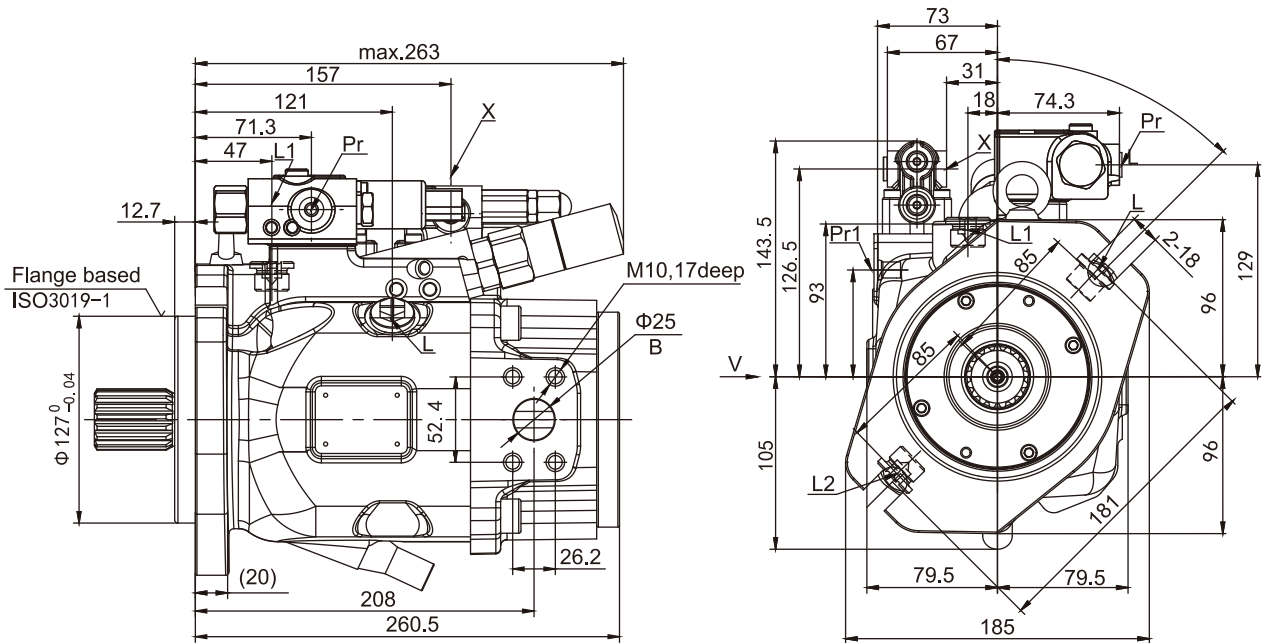
LEDS.-Pressure, Flow, Power controller, mounting flange C, series 01
