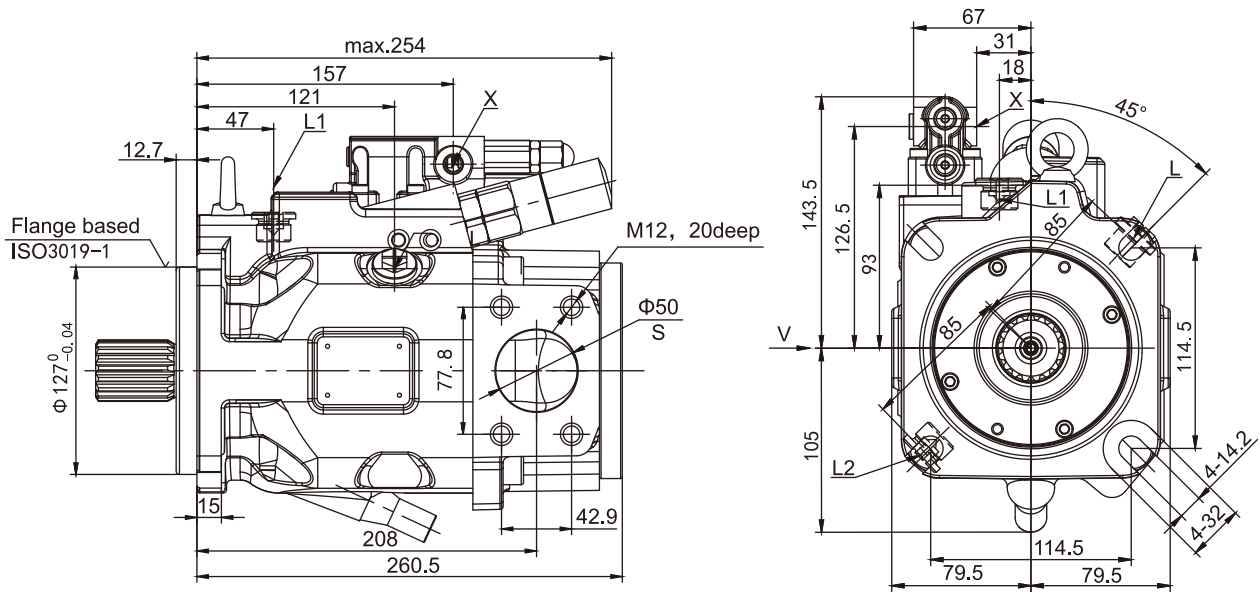
LA.D.-Pressure, Flow, Power controller, mounting flange D, series 01
