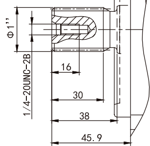
Shaft U
