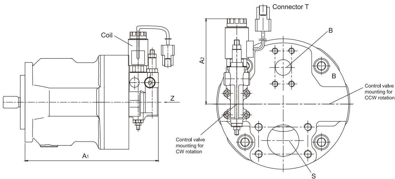
Detail Z
