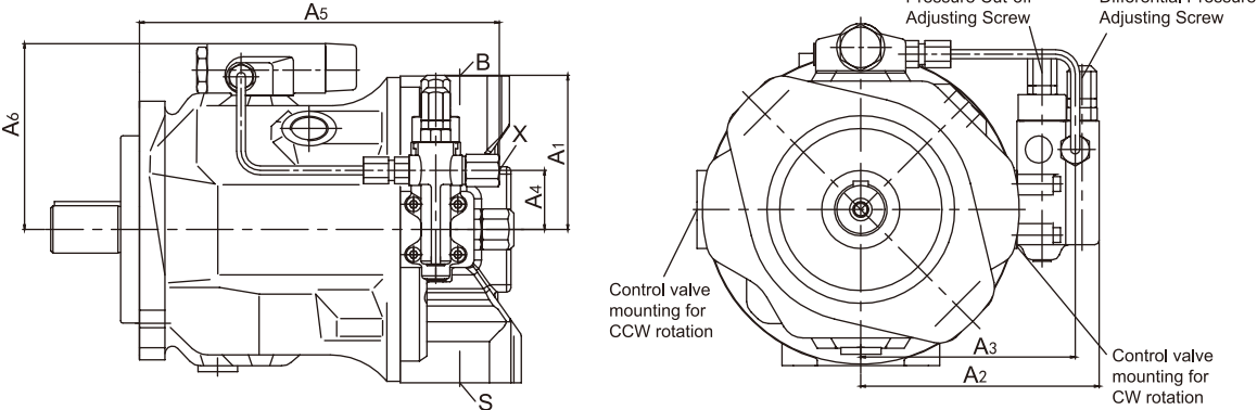
Size 18-110 12N00&62N00
