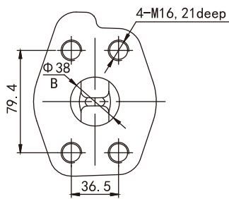
Detail W
