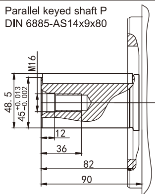
Splined shaft S 2) ANSI B92.1a 30° 1-3/4" 13T 8/16DP
