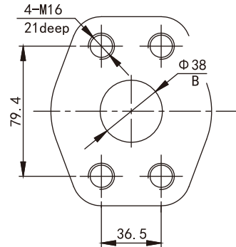
Detail V
