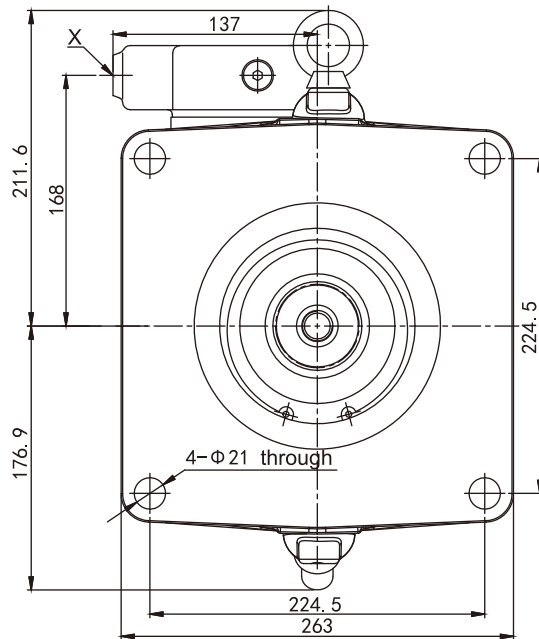
Detail V
