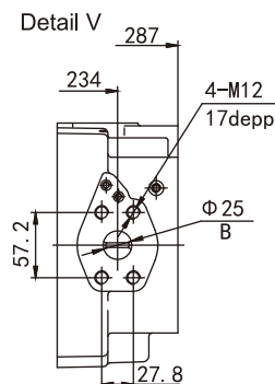
Detail V
