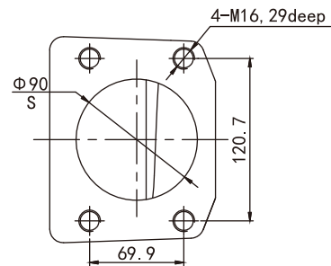
Detail V
