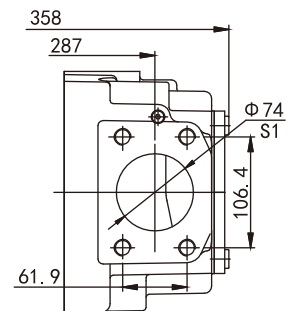
Detail V
