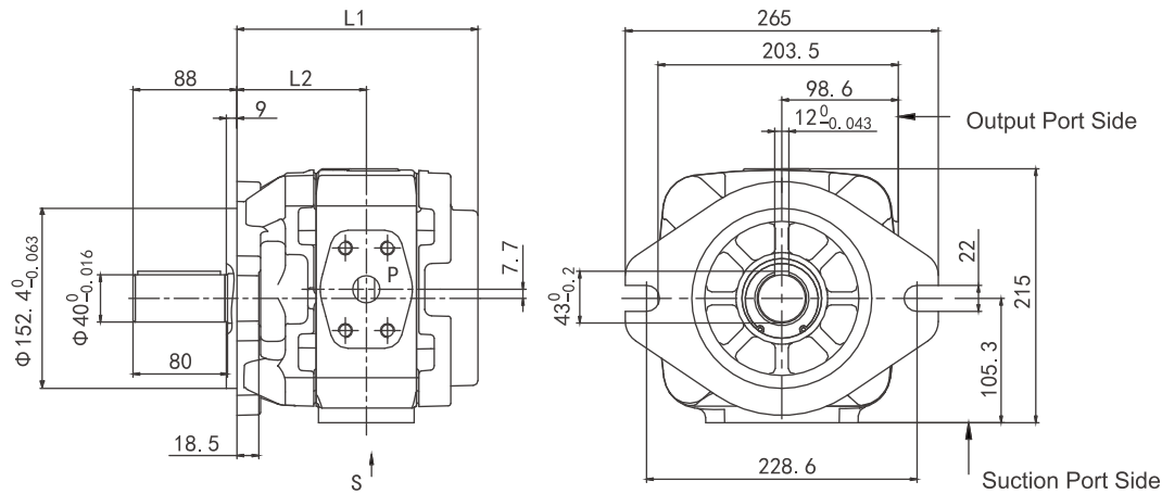
HG2-※-01R-VPC (Parallel keyed shaft)
