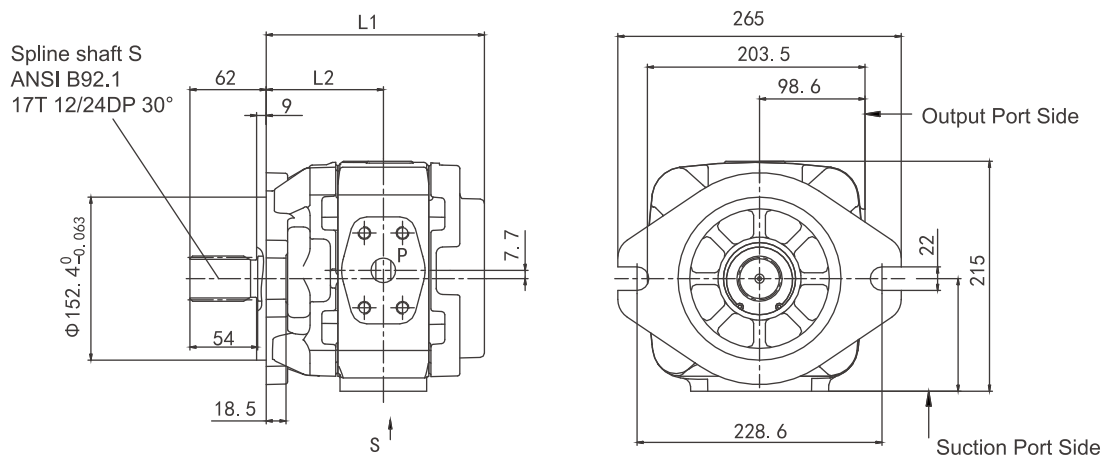
HG2-※-01R-VSC (Spline shaft)
